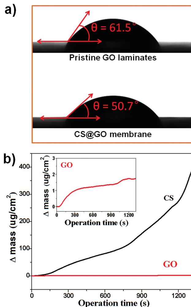
Figure 7. a) Contact angle of the pristine GO laminates and CS@GO membrane. b) Water-sorption ability of CS and GO measured by QCM. The inset is an enlarged figure for the water-sorption ability of GO.
